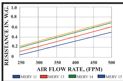
STANDARD PRESSURE DROP Test Filter Size 24" x 24" x 4" Nominal Box
